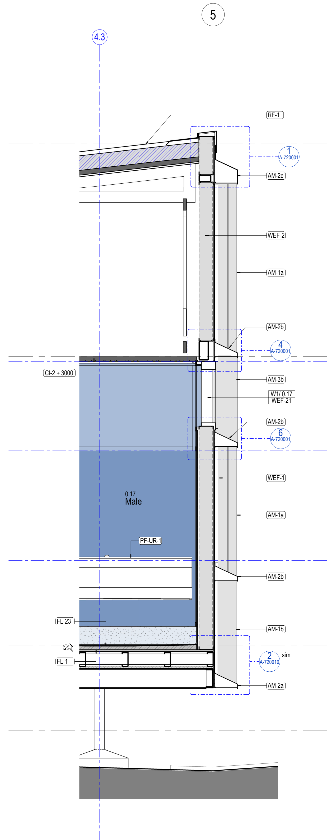
1 South Mid Window Section 1 : 20 Male Amenities
