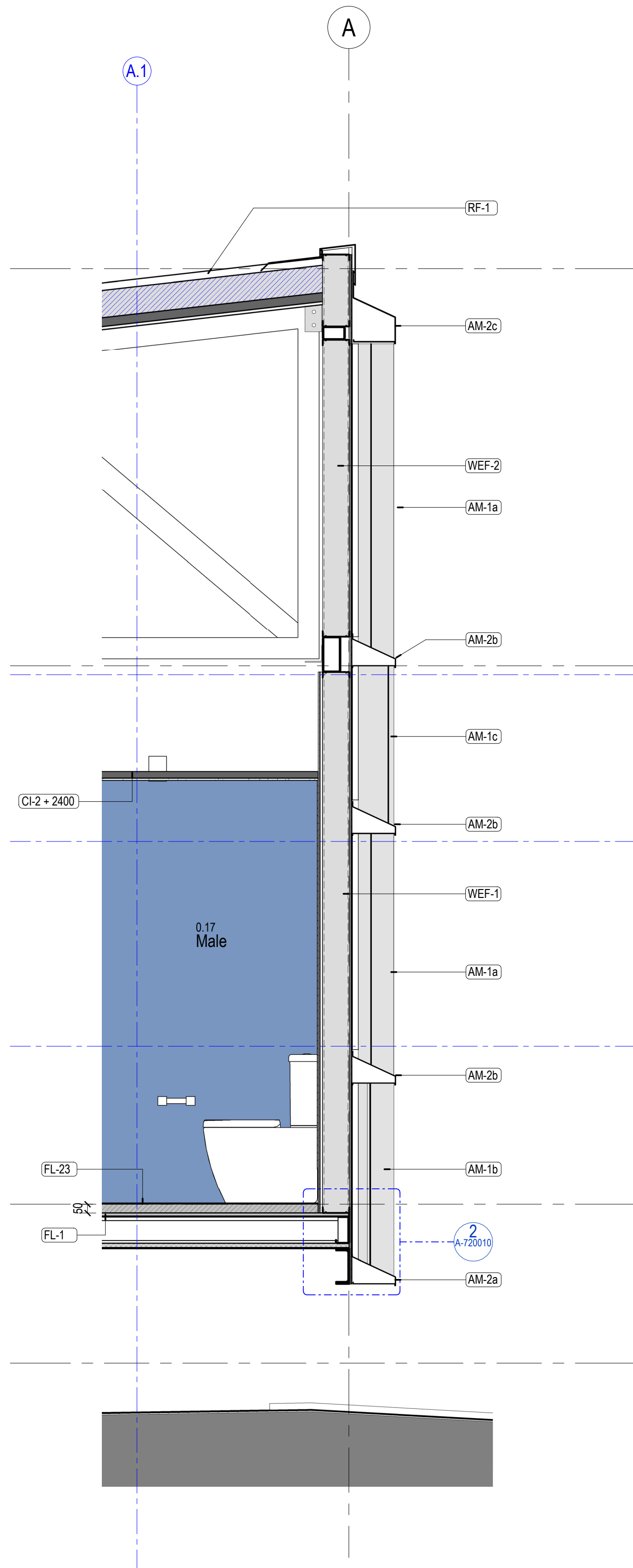
2 West Facade at Set Down Section 1 : 20 Male Amenities
