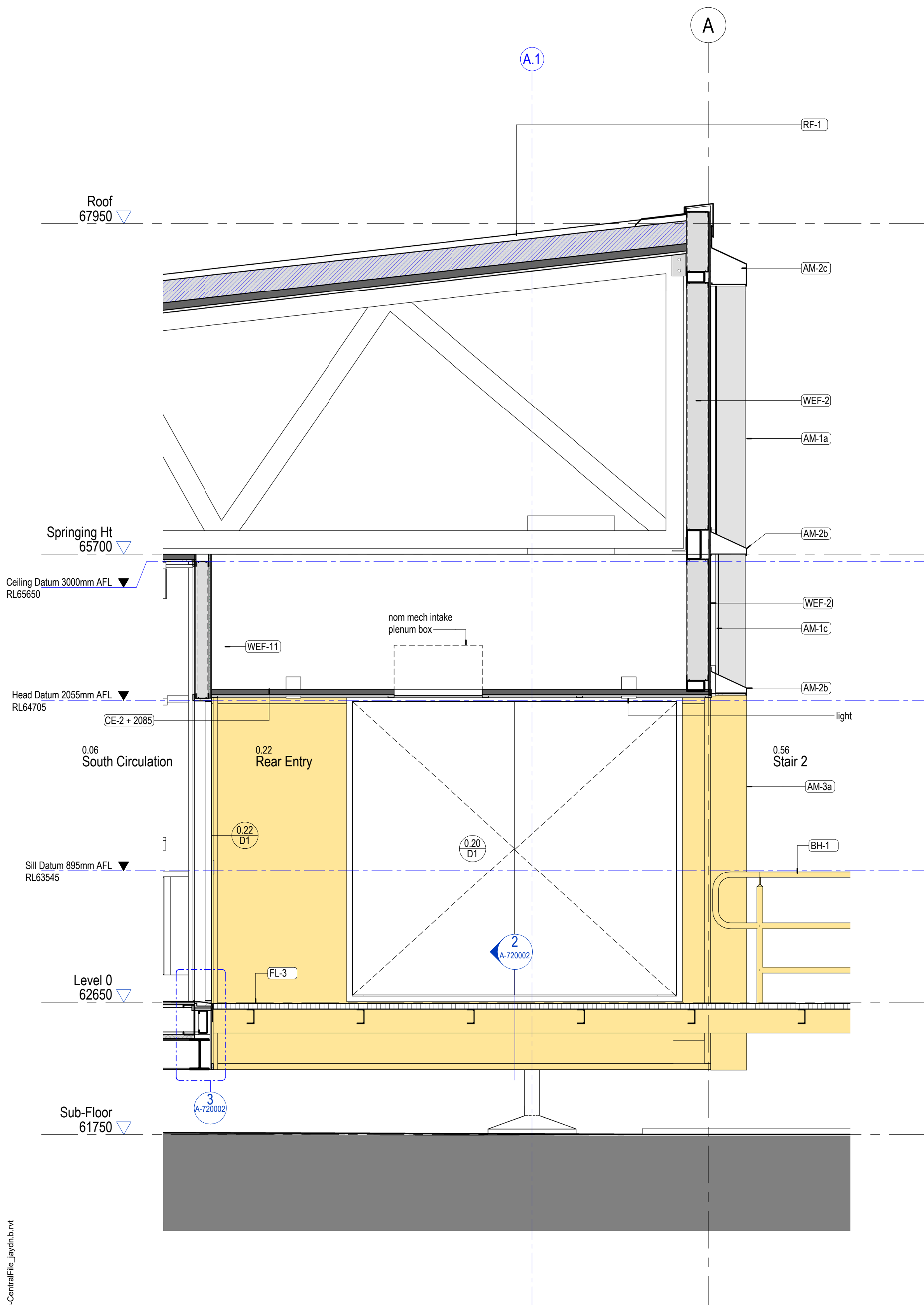
3 West Rear Entry Facade 1 : 20
